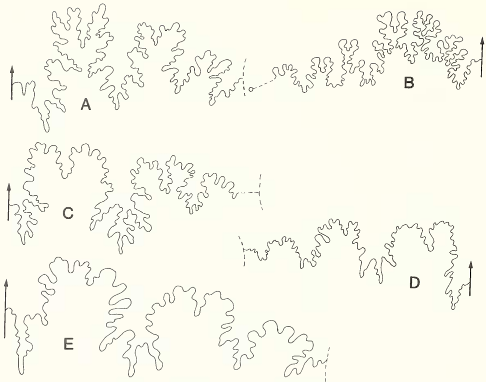
TEXT-FIG. 6. Suture-lines of Kurdistan ammonites. A, Spiticerus (Spiticerus) spathi sp. nov., at 31 mm whorl height; BMNH C.86847; from bed 137; Chia Gara. B, Oxylenticeras lepidum Spath, at 22 mm whorl height; BMNH C.87051; from Chia Gara. C, Euthymiceras kurdistanense sp. nov., at 23 mm whorl height; BMNH C.86825; from bed 137; Chia Gara. D-E, Groebericeras rocardi (Pomel); D, at 32 mm whorl height; BMNH C.86823; from bed 136; Chia Gara; E, at 44 mm whorl height; BMNH C.86936; from bed 46; Banik. A, C-E, \times 2.3 ; B, \times 3.4 .
